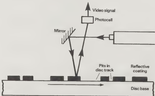
The inner workings of a Philips LaserVision videodisc player.
